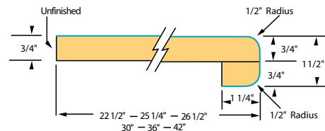
FLAT DECK TOP EWFV-22 1/2 EWFK-25 1/4 EWFB-26 1/2 EWF-30 EWF-36 EWF-42
