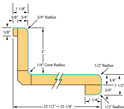
KITCHEN AND VANITY EWW-22 1/2 EWK- 25 1/4
